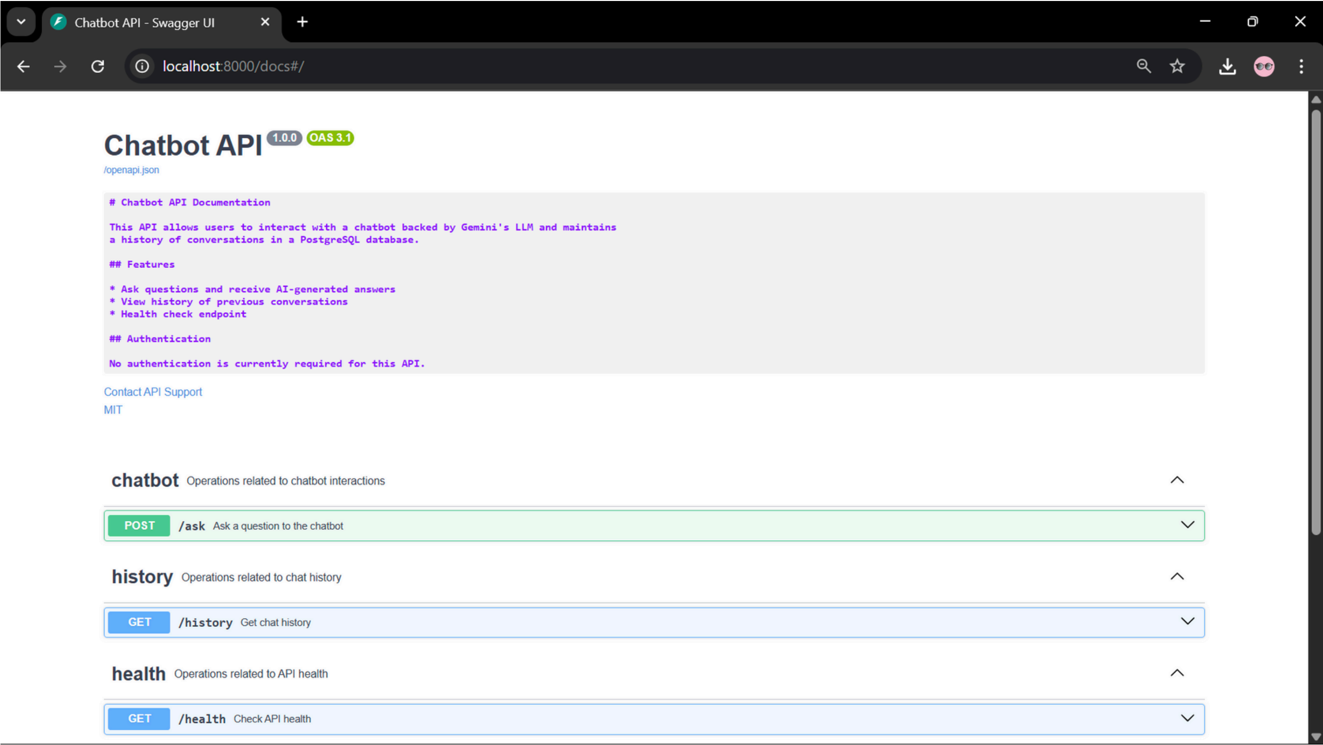
Swagger UI
